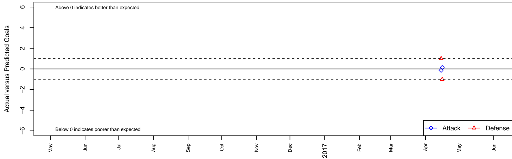
Warriors SC Denam B02 Dots are actual minus expected GF (blue circles) and GA (red triangles). Blue line is smoothed change in attack strength. Red is smoothed change in defense strength.
